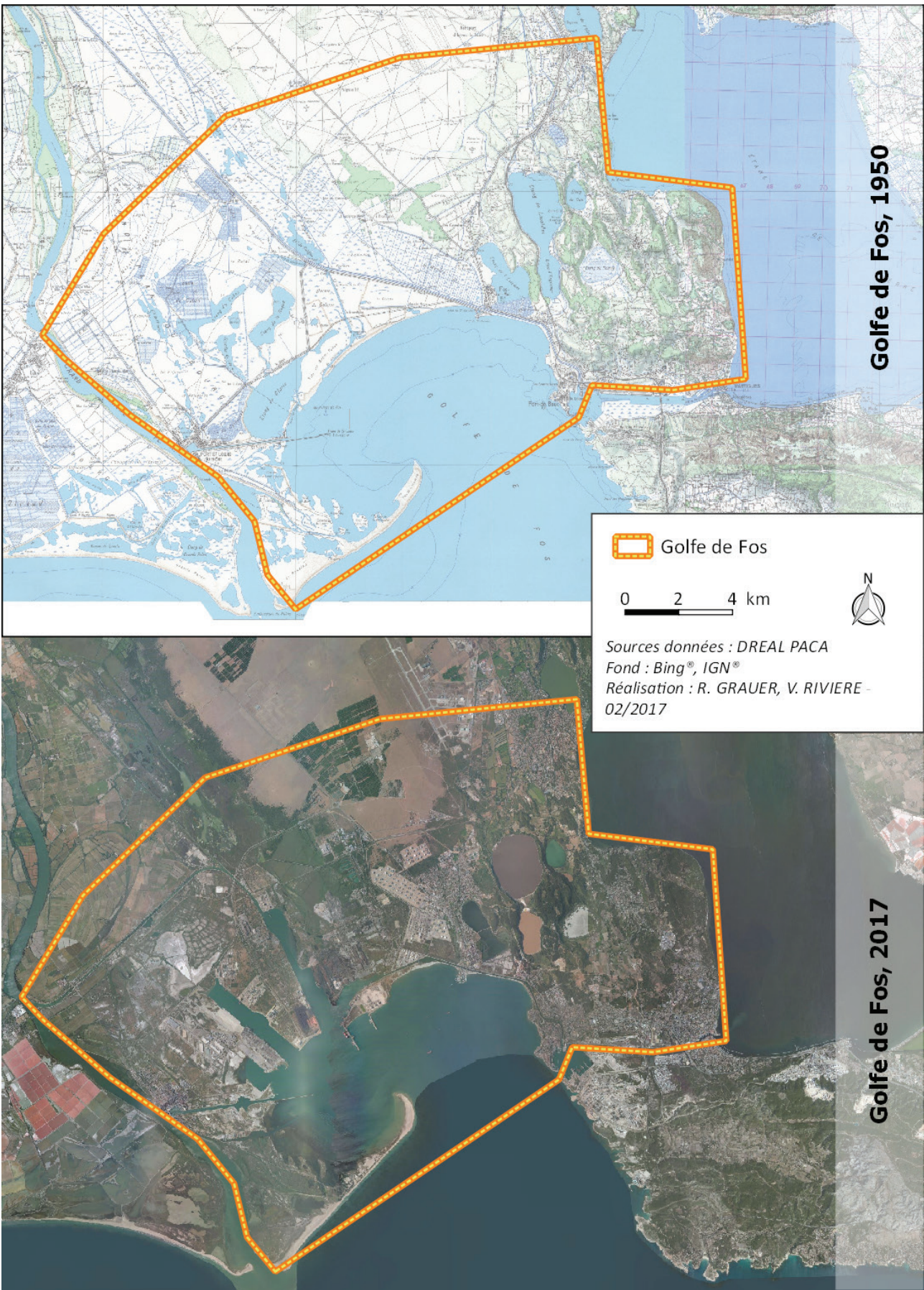
Figure 8 : : Comparaison des modifications du Golfe du Fos entre 1950 (avant le développement portuaire) et 2017. Figure 8: Comparison of changes between 1950 (before the port was developed) and 2017 in the Gulf of Fos.
